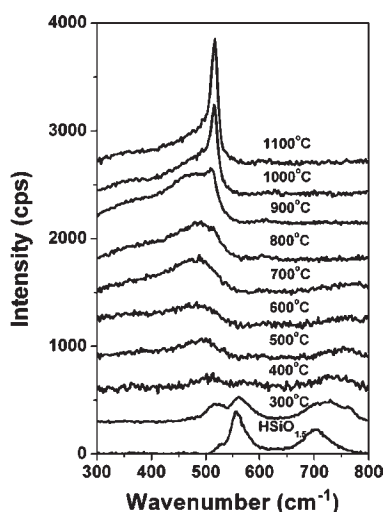
Figure 3. Thermal transformation of meso- \text{HSiO}_{1.5} to meso-ncSi/ \text{SiO}_2 . Evolution of the Raman spectrum of meso- \text{HSiO}_{1.5} as a function of heating from 300 to 1100 °C under a slightly reducing atmosphere (5% \text{H}_2 /95% Ar).
